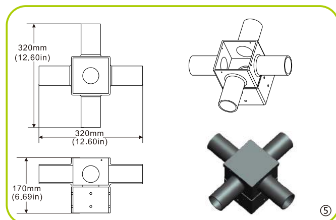
⑤ 4 lights square rod adapter
