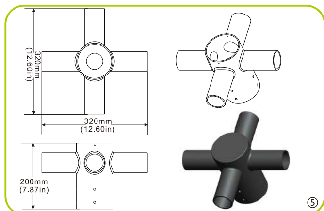
⑤ 4 lights round rod adapter
