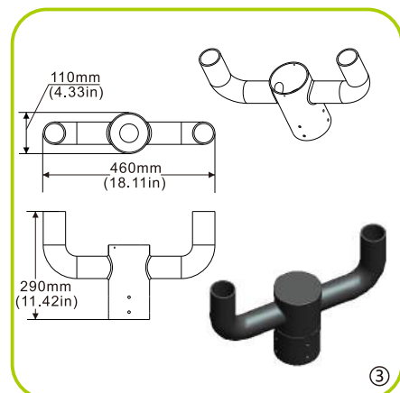
③ 2 opposite lights round rod bending joint
