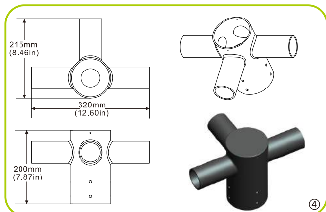
④ 3 lights round rod adapter
