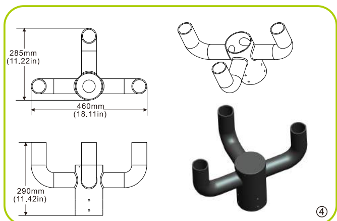
④ 3 lights round rod bending joint
