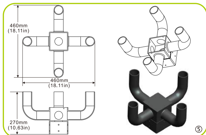
⑤ 4 lights square rod bending joint
