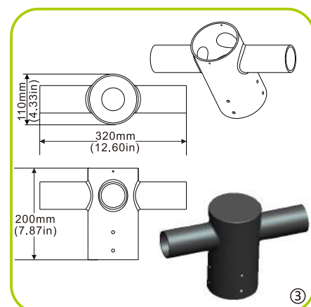
③ 2 opposite lights round rod adapter
