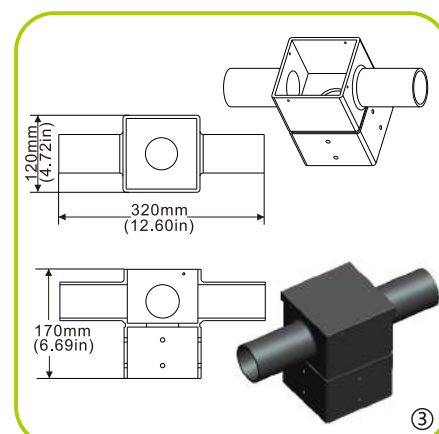
③ 2 opposite lights square rod adapter
