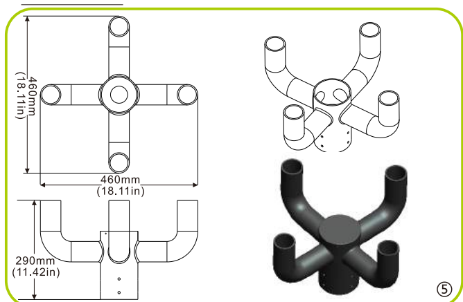
⑤ 4 lights round rod bending joint
