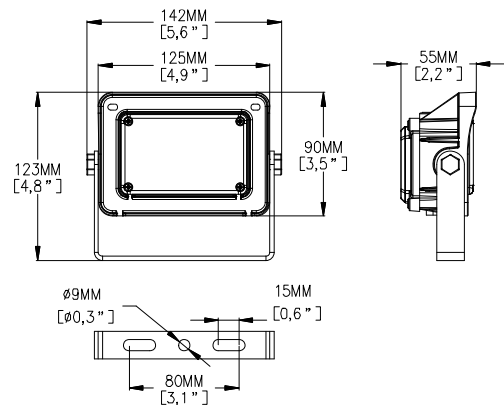
"U" YOKE Bracket 0.5kg(1.1lbs)
