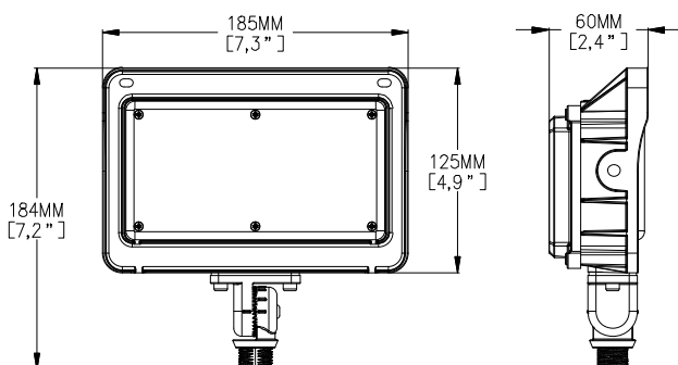
½ NTSM Knuckle Mount 1.0kg(2.2lbs)
